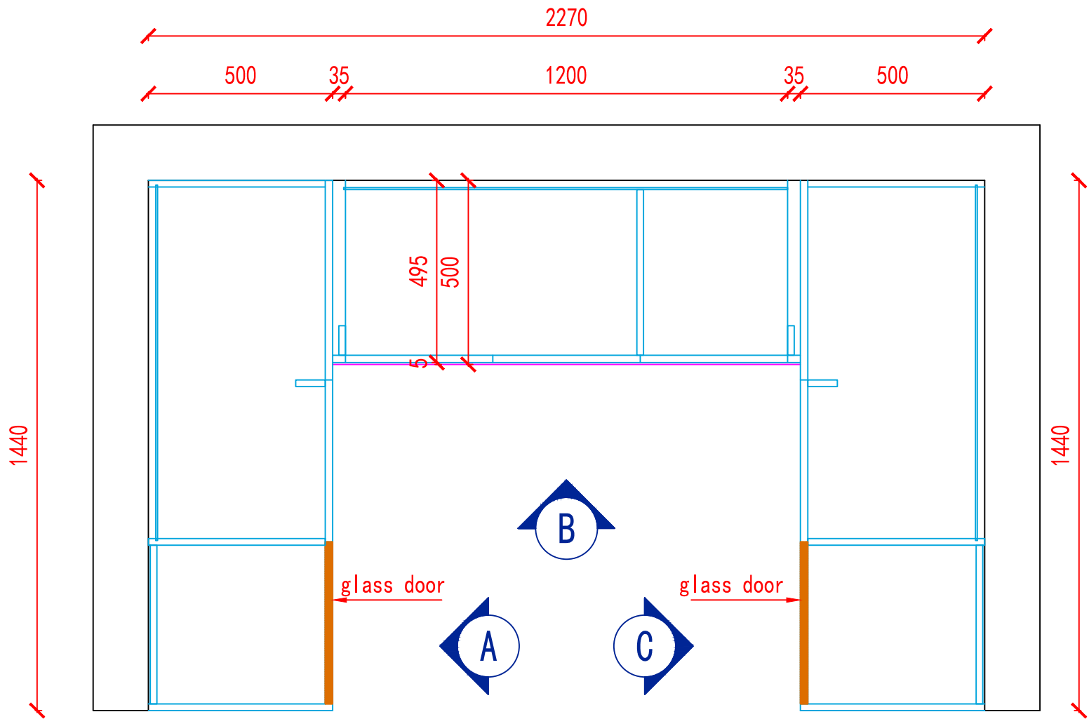
basic cabinet plan
